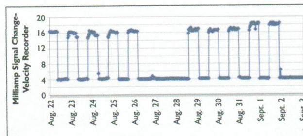
Figure 2: SF-9 air velocity increase before/after cleaning.
